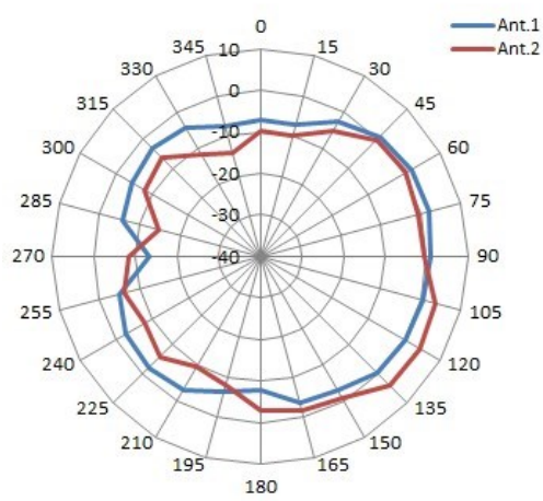
2.4GHz Azimuth-Plane
