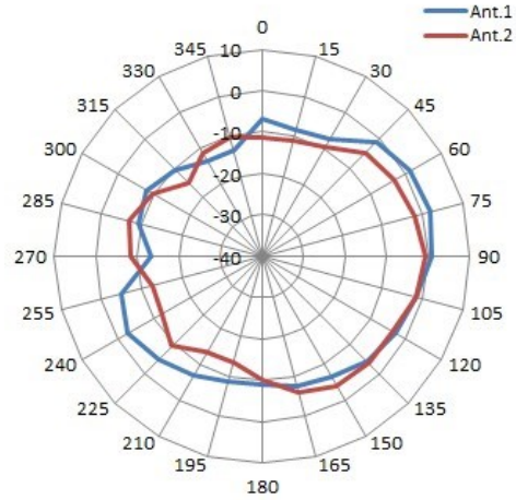
2.4GHz Elevation-Plane
