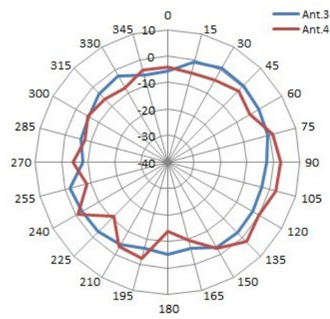
5GHz Azimuth-Plane
