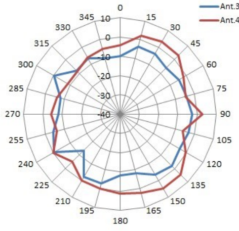
5GHz Elevation-Plane
