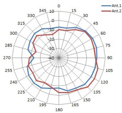
2.4GHz Azimuth-Plane
